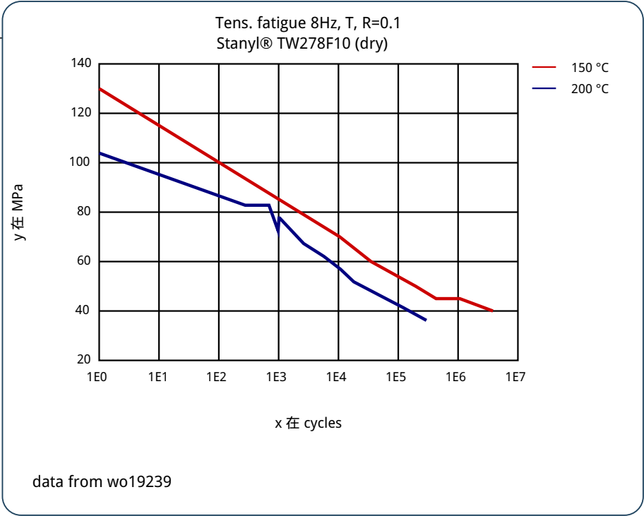
Tens. fatigue 8Hz, T, R=0.1 , dry
